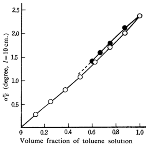
Fig. 3. Changes in optical rotation with the addition of n -heptane ( \circ ) and n -butanol ( \bullet ) to 1.05% solution of poly- l -4-methyl-1-hexene in toluene. Dotted line, precipitation occurred.
