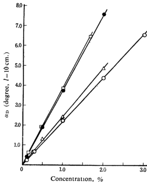
Fig. 1. Optical rotation vs. concentration of poly- l -4-methyl-1-hexene in various solvents: \circ in toluene at 27.5^\circ\text{C} ; \triangle in decalin at 24^\circ\text{C} ; \square in carbon tetrachloride at 25^\circ\text{C} ; \bullet in carbon disulfide at 13^\circ\text{C} .
